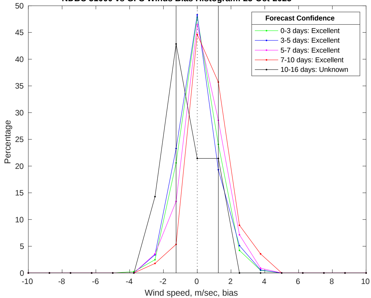
NDBC 51000 vs GFS Winds Bias Histogram: 25-Oct-2025
