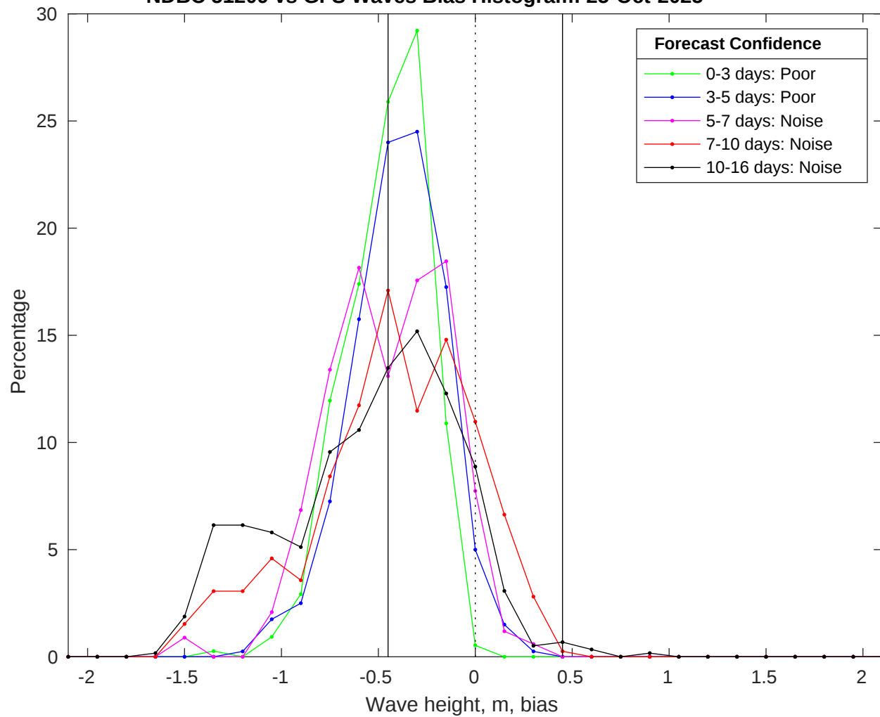
NDBC 51209 vs GFS Waves Bias Histogram: 25-Oct-2025
