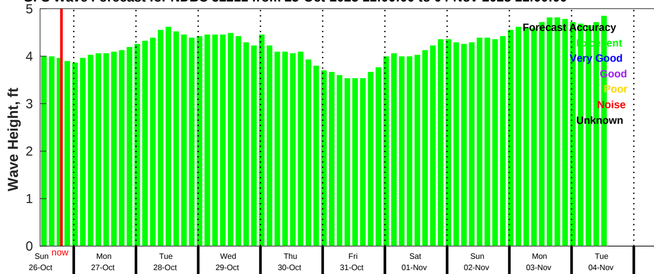
GFS Wave Forecast for NDBC 52211 from 25-Oct-2025 11:00:00 to 04-Nov-2025 11:00:00
