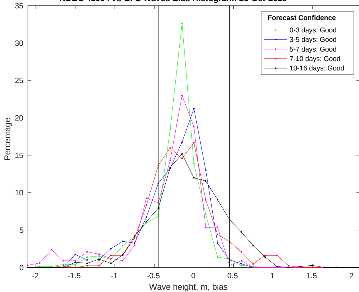
NDBC 41004 vs GFS Waves Bias Histogram: 26-Oct-2025
