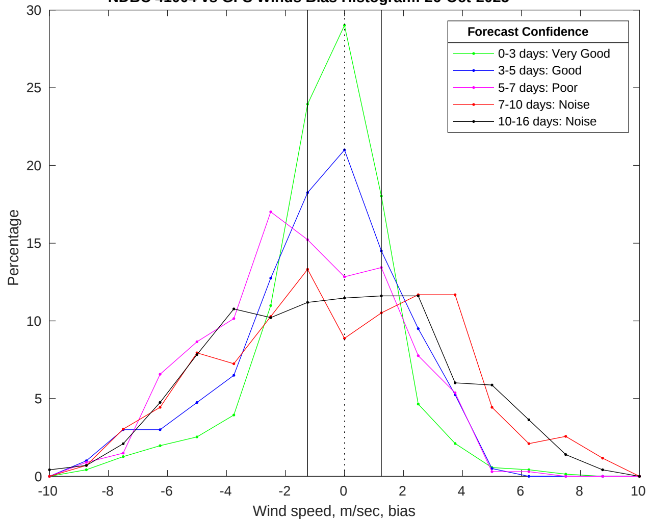
NDBC 41004 vs GFS Winds Bias Histogram: 26-Oct-2025
