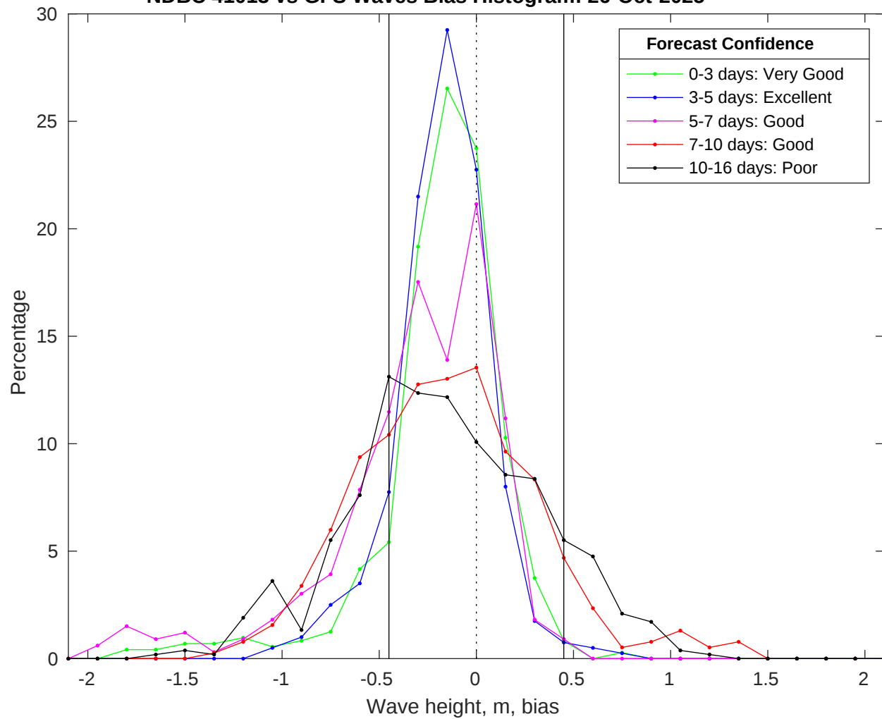
NDBC 41013 vs GFS Waves Bias Histogram: 26-Oct-2025
