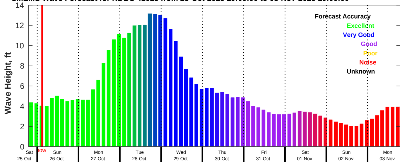
CMEMS Wave Forecast for NDBC 41013 from 25-Oct-2025 19:00:00 to 03-Nov-2025 19:00:00
