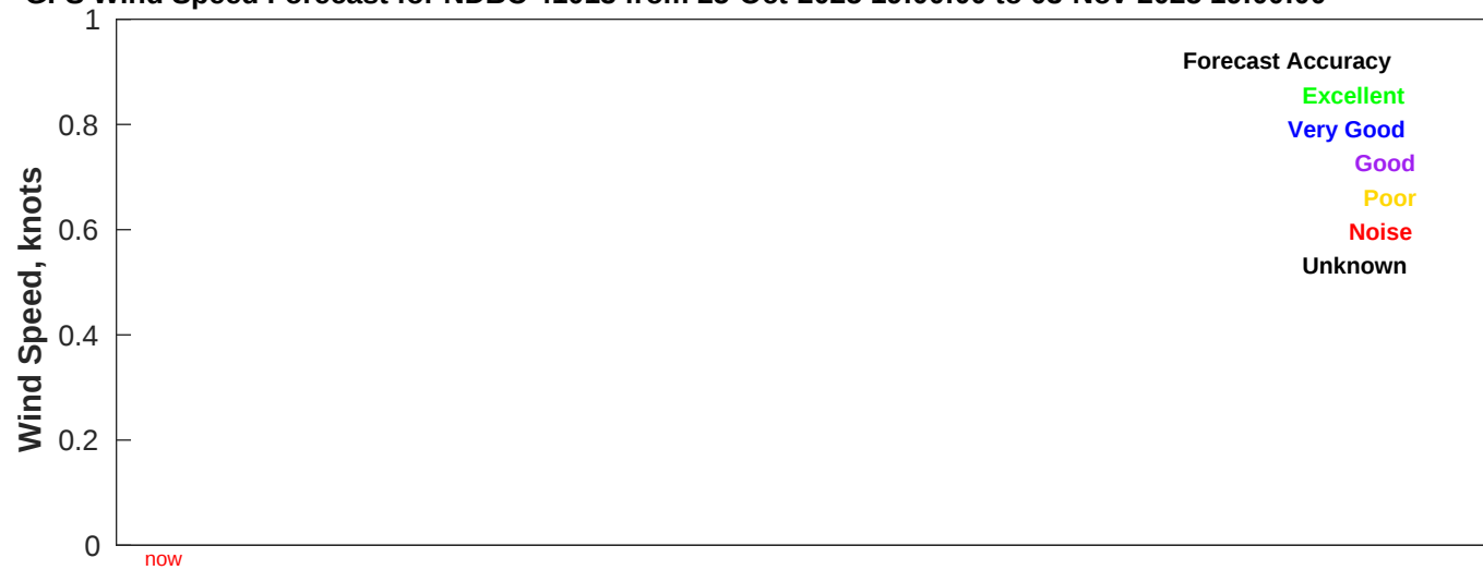
GFS Wind Speed Forecast for NDBC 41013 from 25-Oct-2025 19:00:00 to 03-Nov-2025 19:00:00
