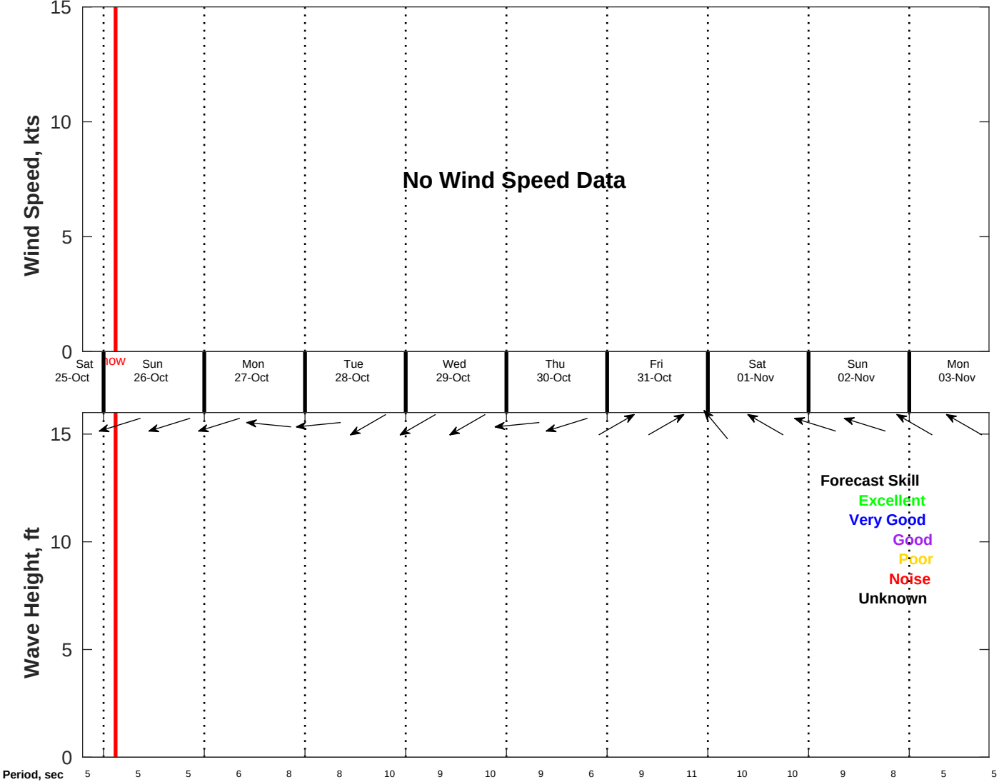
Wind & Wave Forecast for NDBC 41013 from 25-Oct-2025 19:00:00 to 03-Nov-2025 19:00:00
