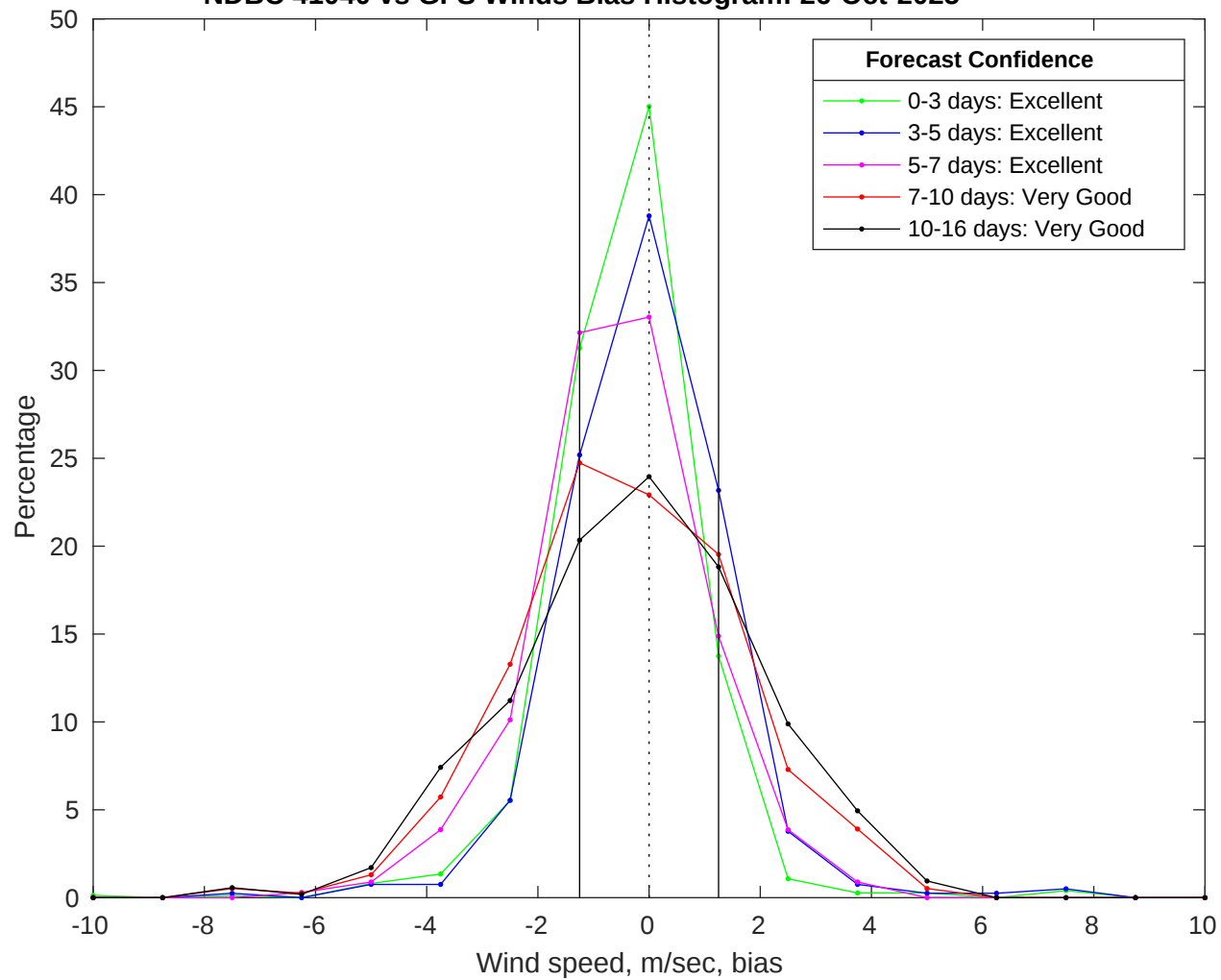
NDBC 41040 vs GFS Winds Bias Histogram: 26-Oct-2025
