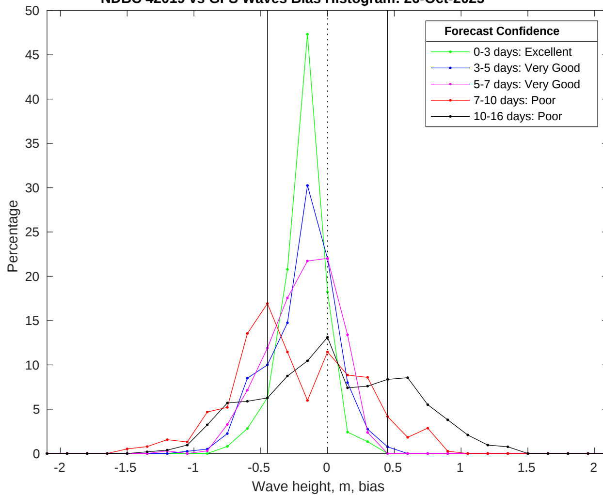
NDBC 42019 vs GFS Waves Bias Histogram: 26-Oct-2025
