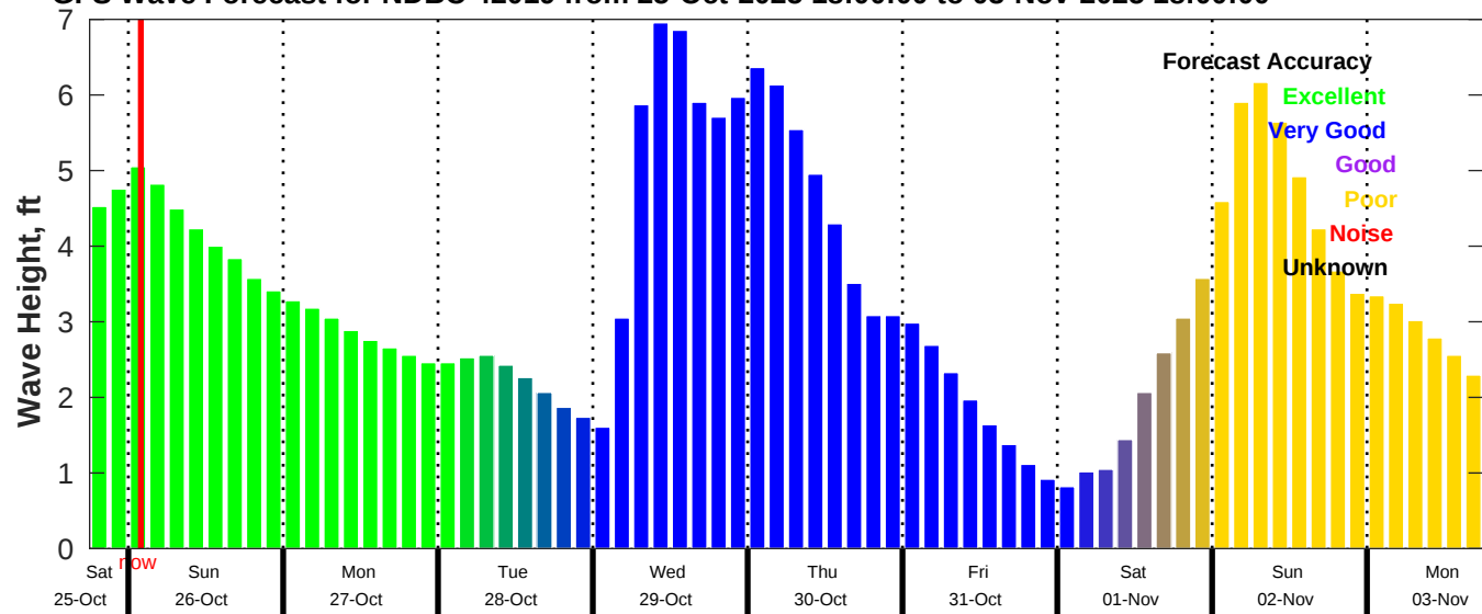
GFS Wave Forecast for NDBC 42019 from 25-Oct-2025 18:00:00 to 03-Nov-2025 18:00:00
