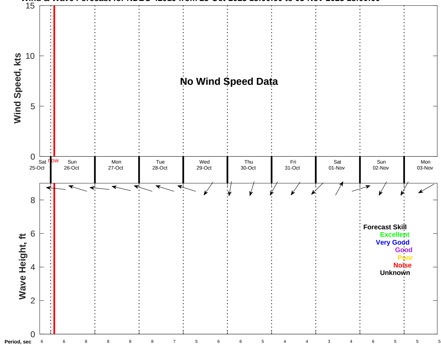
Wind & Wave Forecast for NDBC 42019 from 25-Oct-2025 18:00:00 to 03-Nov-2025 18:00:00
