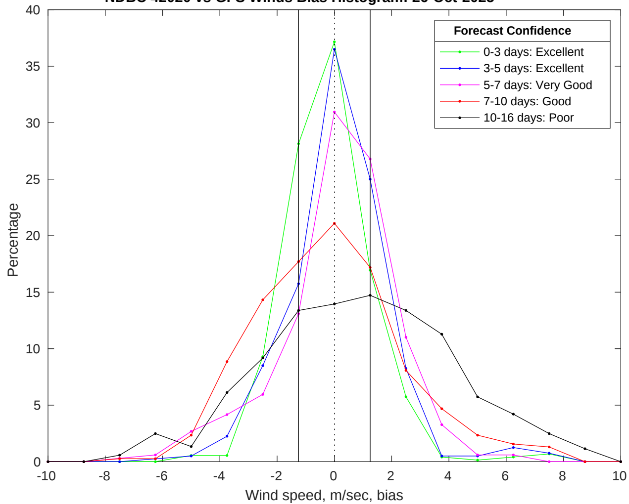
NDBC 42020 vs GFS Winds Bias Histogram: 26-Oct-2025
