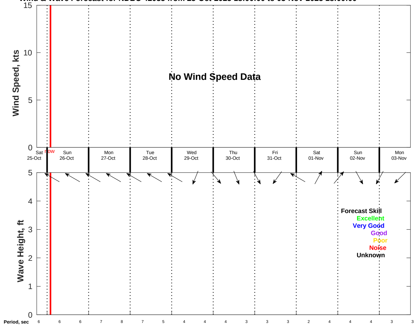
Wind & Wave Forecast for NDBC 42035 from 25-Oct-2025 18:00:00 to 03-Nov-2025 18:00:00
