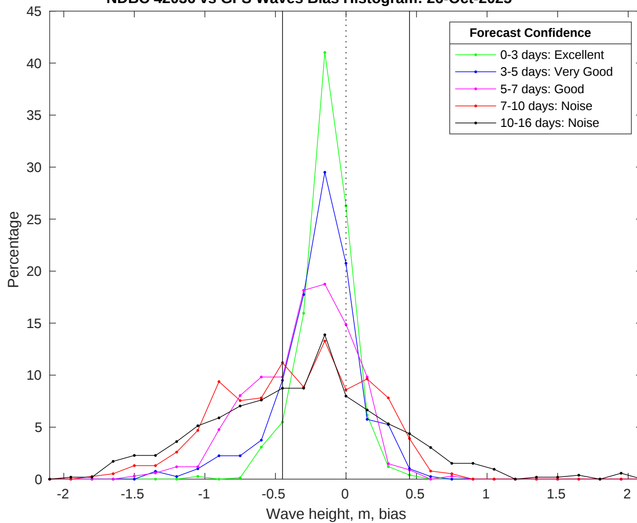
NDBC 42036 vs GFS Waves Bias Histogram: 26-Oct-2025
