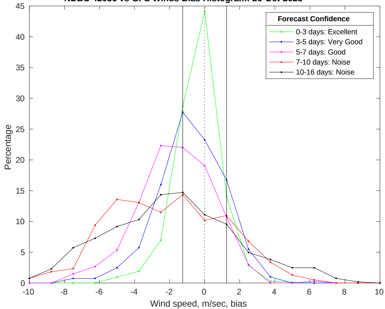
NDBC 42036 vs GFS Winds Bias Histogram: 26-Oct-2025
