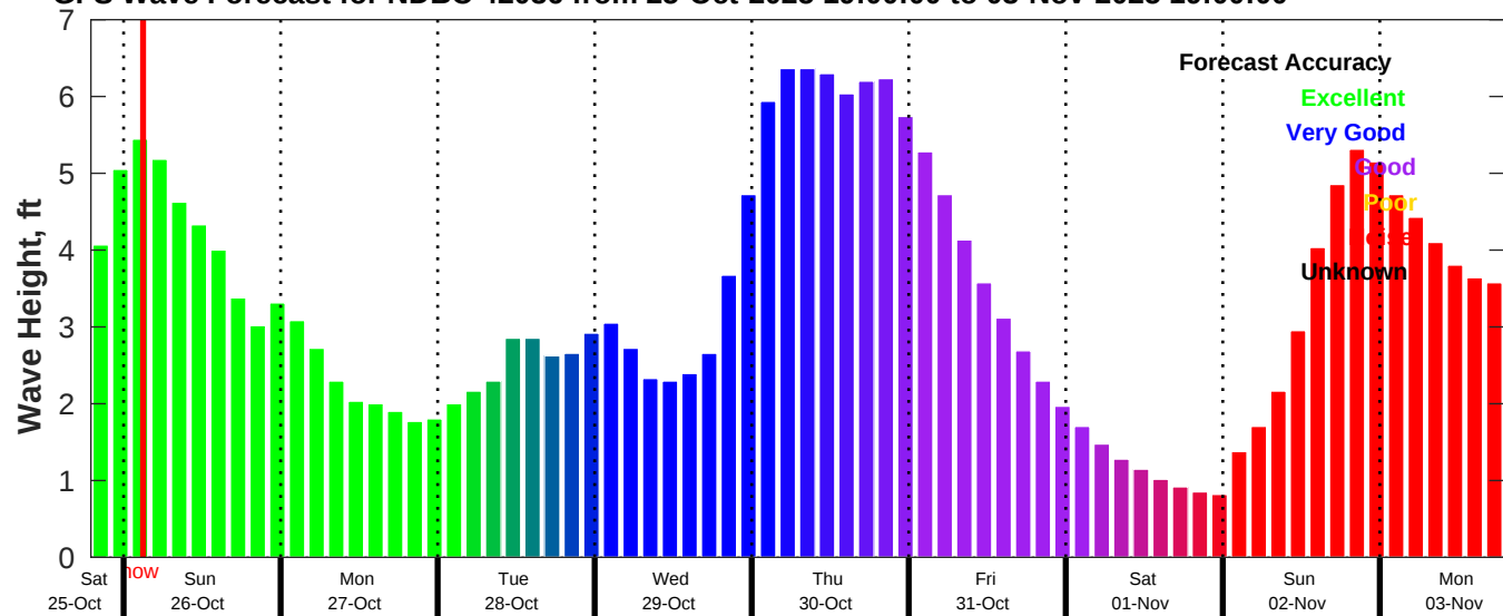
GFS Wave Forecast for NDBC 42036 from 25-Oct-2025 19:00:00 to 03-Nov-2025 19:00:00
