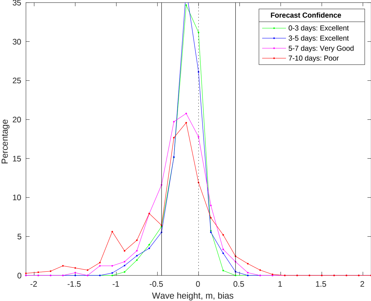
NDBC 42040 vs CMEMS Waves Bias Histogram: 26-Oct-2025
