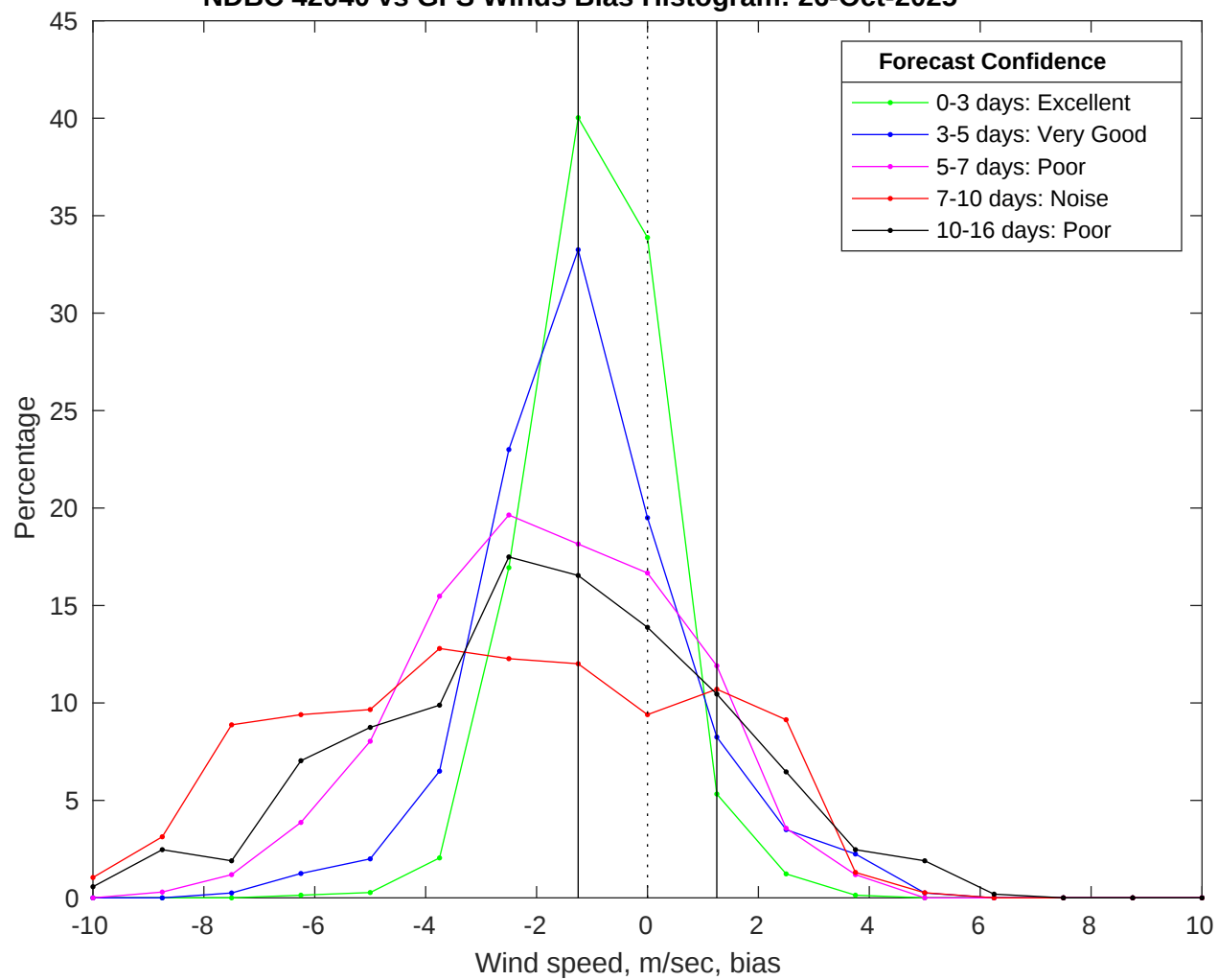
NDBC 42040 vs GFS Winds Bias Histogram: 26-Oct-2025
