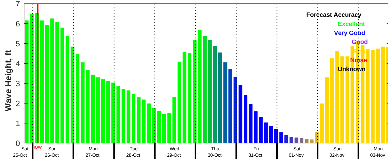
CMEMS Wave Forecast for NDBC 42040 from 25-Oct-2025 19:00:00 to 03-Nov-2025 19:00:00
