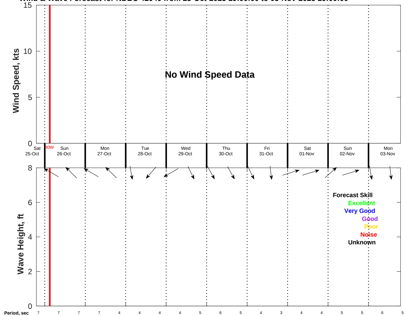
Wind & Wave Forecast for NDBC 42040 from 25-Oct-2025 19:00:00 to 03-Nov-2025 19:00:00
