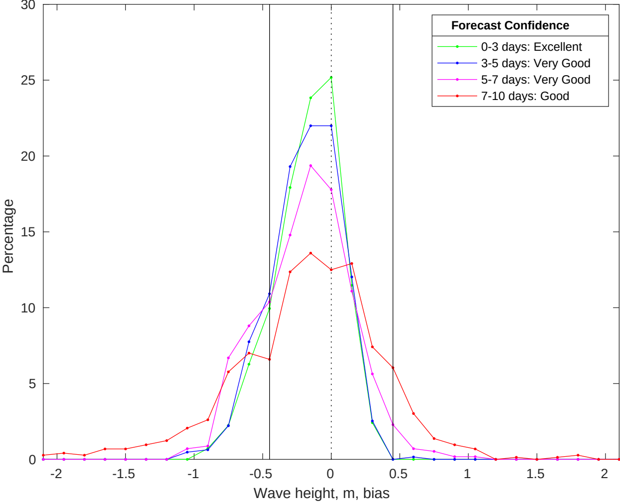
NDBC 46011 vs CMEMS Waves Bias Histogram: 26-Oct-2025
