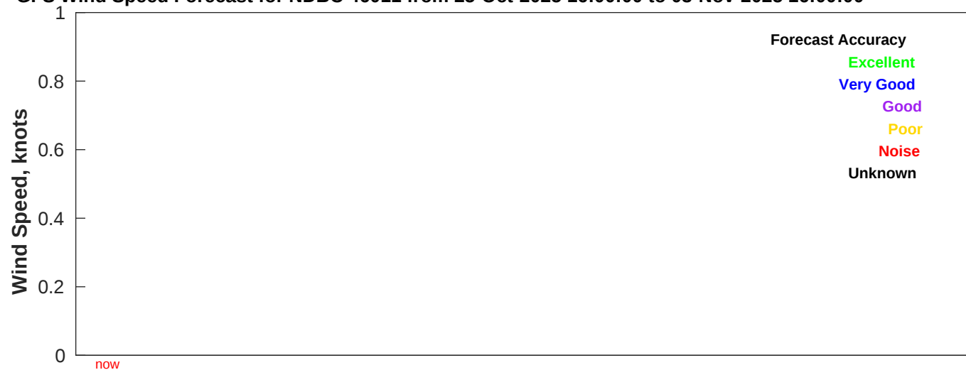
GFS Wind Speed Forecast for NDBC 46011 from 25-Oct-2025 16:00:00 to 03-Nov-2025 16:00:00
