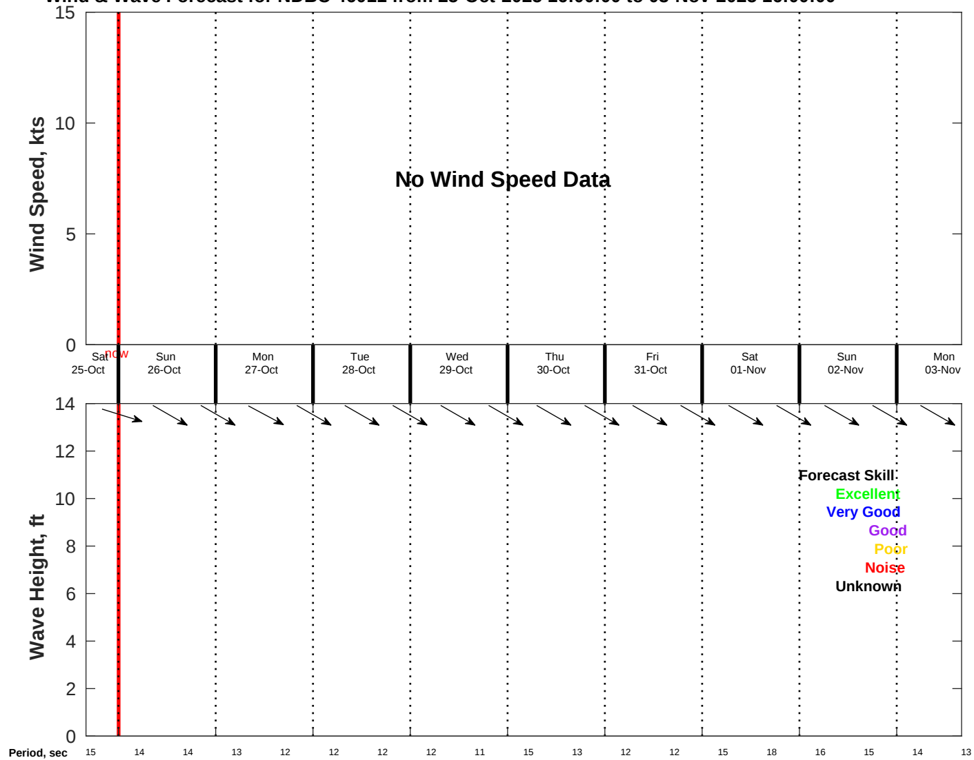
Wind & Wave Forecast for NDBC 46011 from 25-Oct-2025 16:00:00 to 03-Nov-2025 16:00:00
