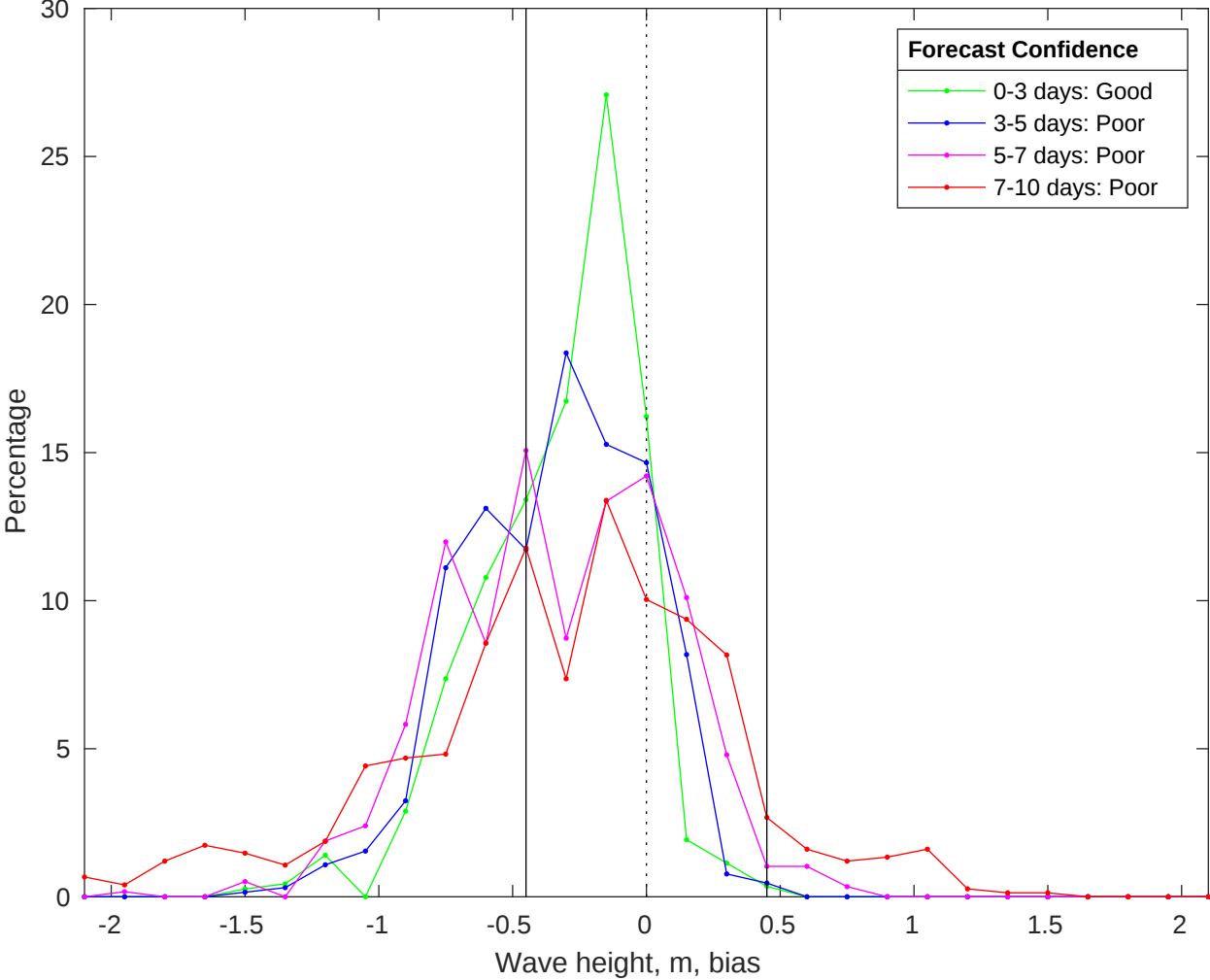
NDBC 46028 vs CMEMS Waves Bias Histogram: 26-Oct-2025
