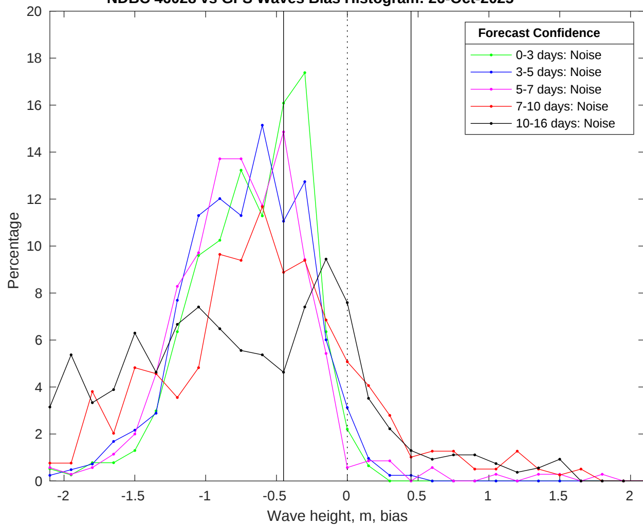
NDBC 46028 vs GFS Waves Bias Histogram: 26-Oct-2025
