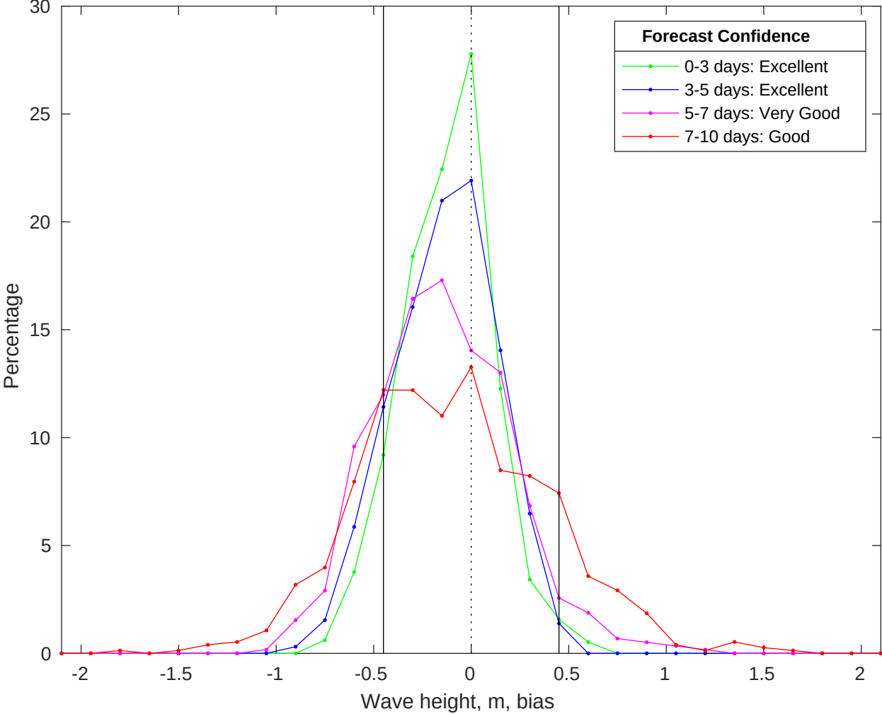
NDBC 46054 vs CMEMS Waves Bias Histogram: 26-Oct-2025
