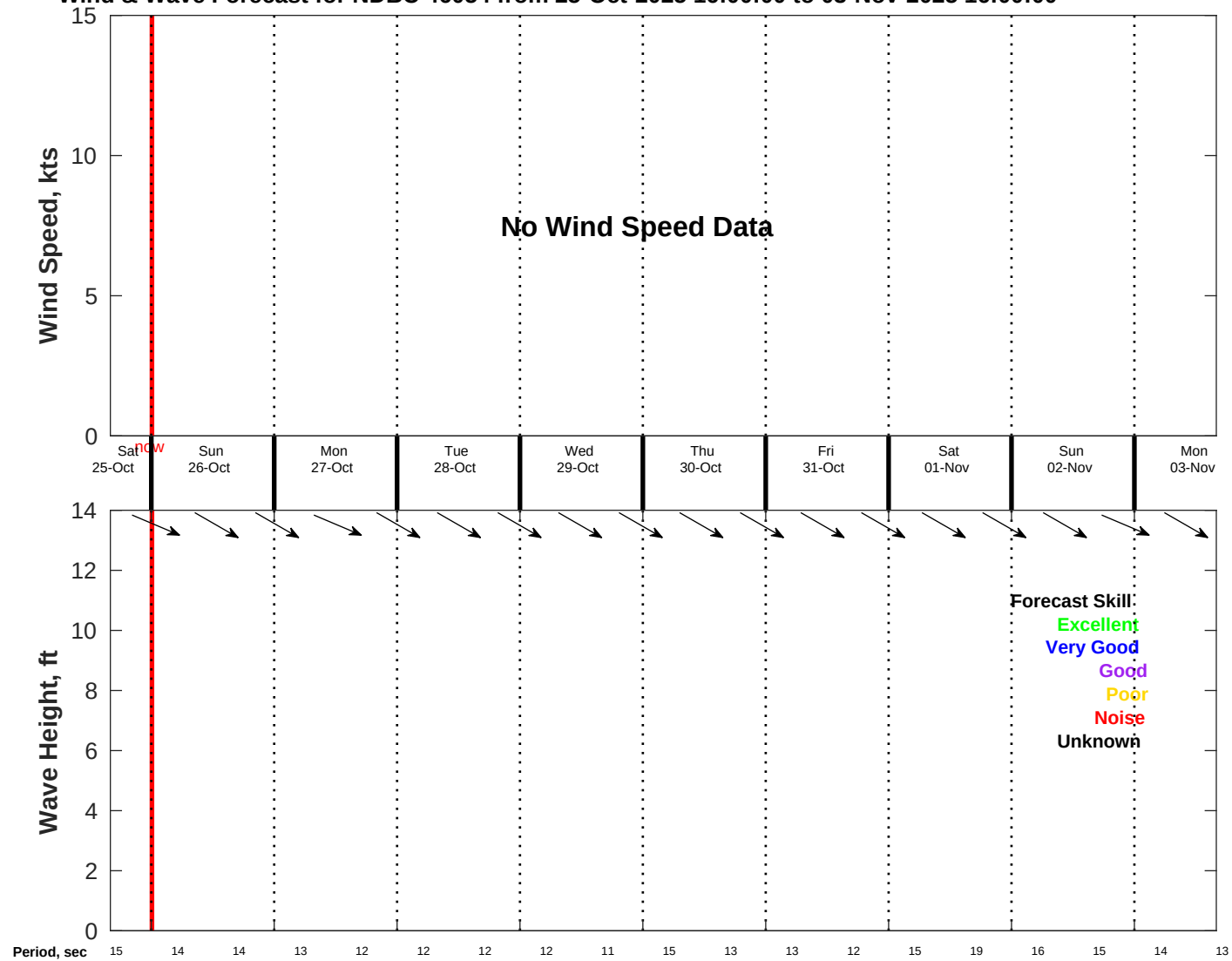
Wind & Wave Forecast for NDBC 46054 from 25-Oct-2025 16:00:00 to 03-Nov-2025 16:00:00
