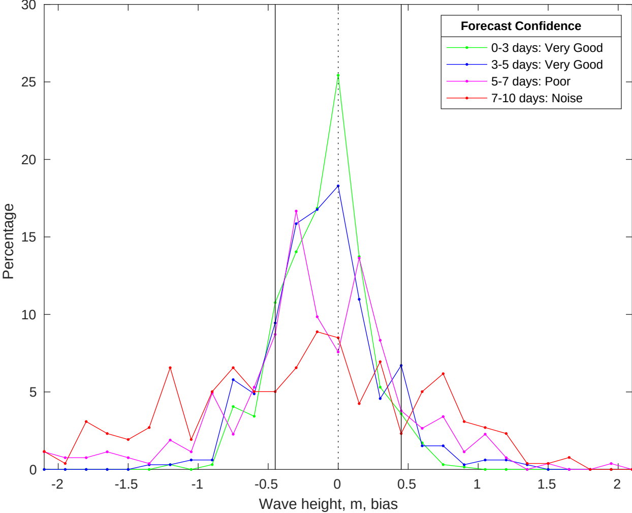
NDBC 46059 vs CMEMS Waves Bias Histogram: 26-Oct-2025
