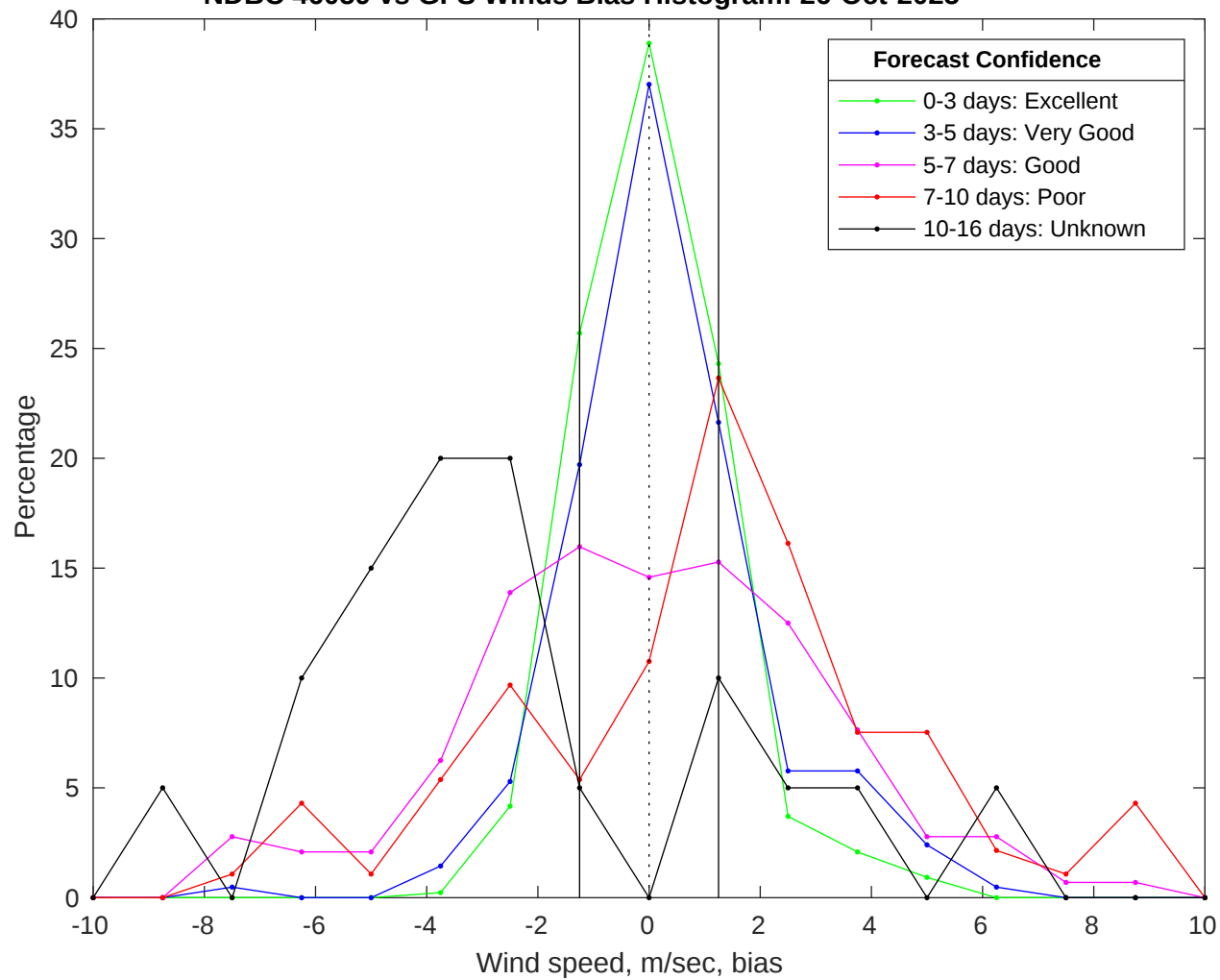
NDBC 46059 vs GFS Winds Bias Histogram: 26-Oct-2025
