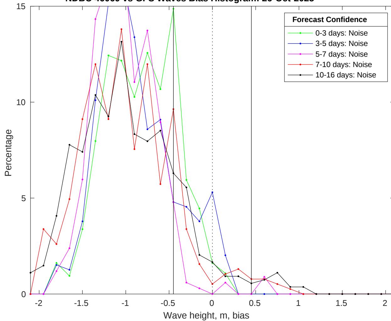
NDBC 46069 vs GFS Waves Bias Histogram: 26-Oct-2025
