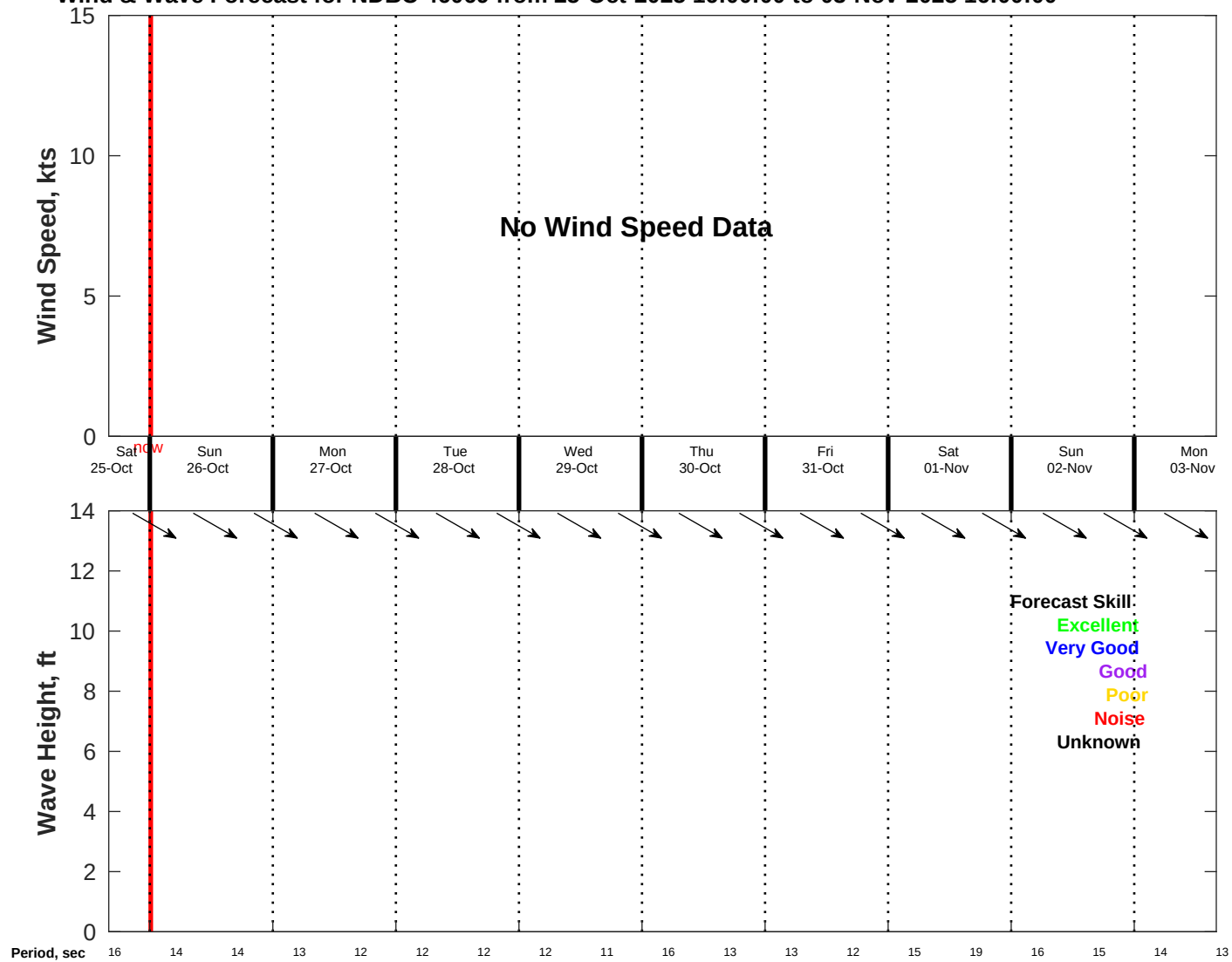
Wind & Wave Forecast for NDBC 46069 from 25-Oct-2025 16:00:00 to 03-Nov-2025 16:00:00
