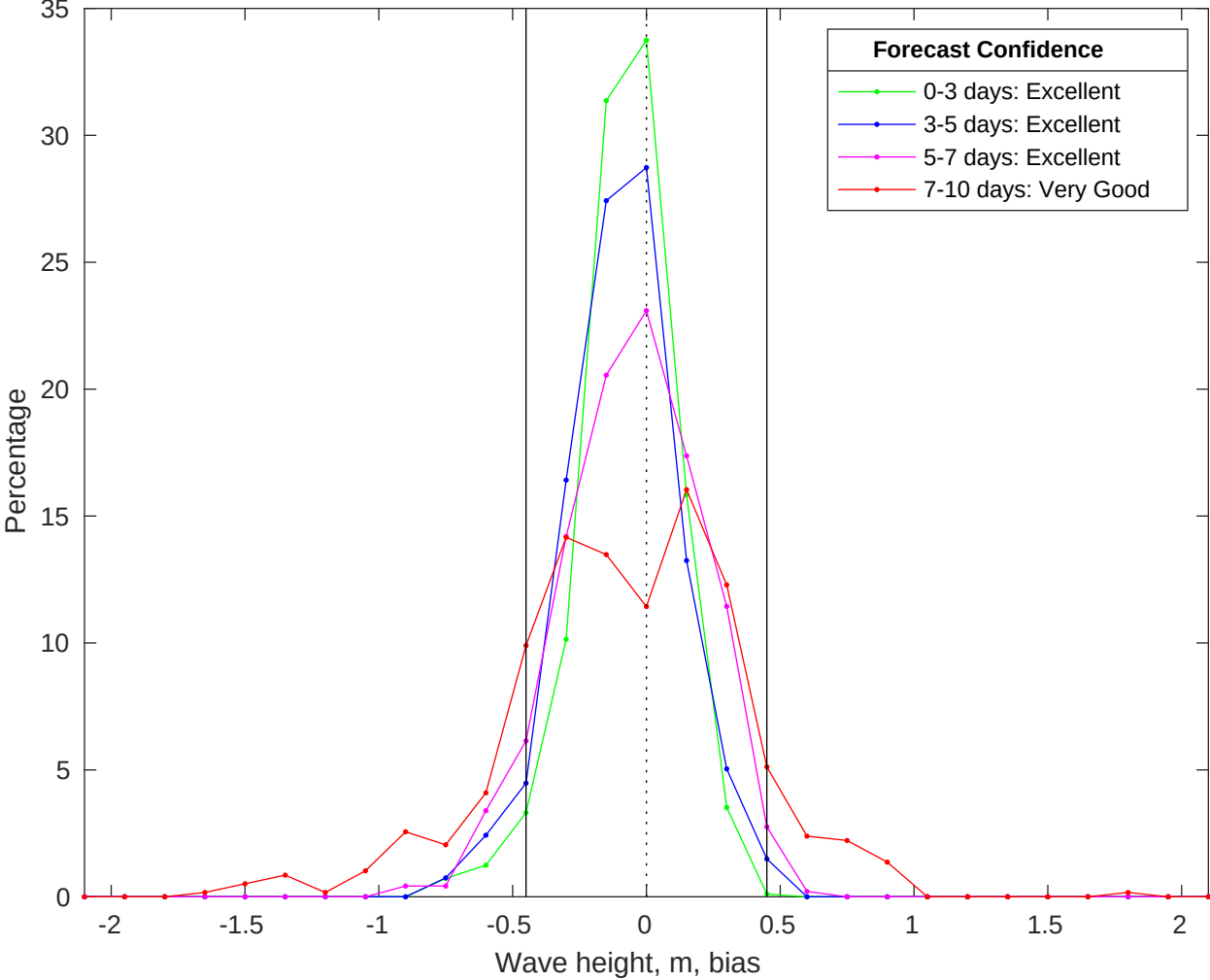
NDBC 46215 vs CMEMS Waves Bias Histogram: 26-Oct-2025
