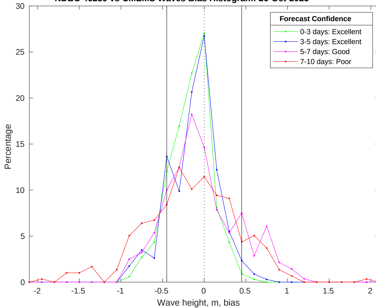
NDBC 46259 vs CMEMS Waves Bias Histogram: 26-Oct-2025
