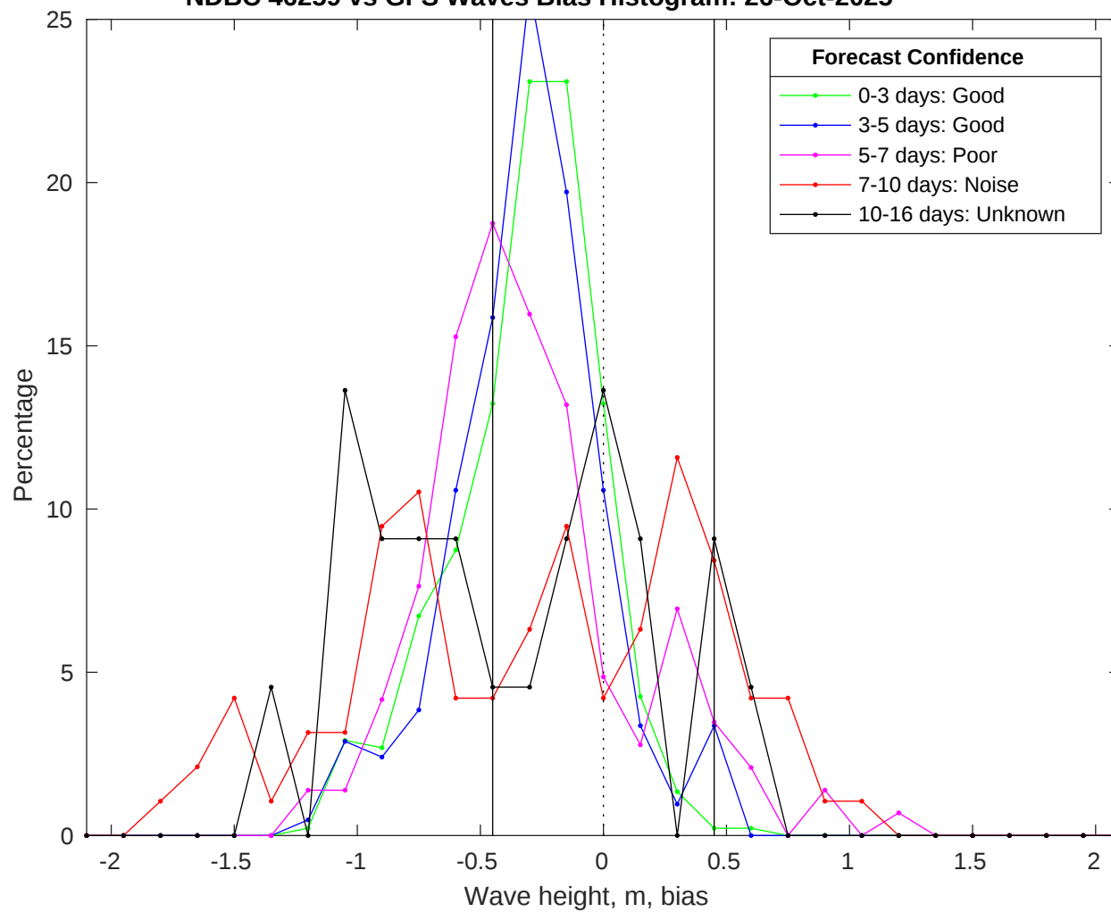
NDBC 46259 vs GFS Waves Bias Histogram: 26-Oct-2025
