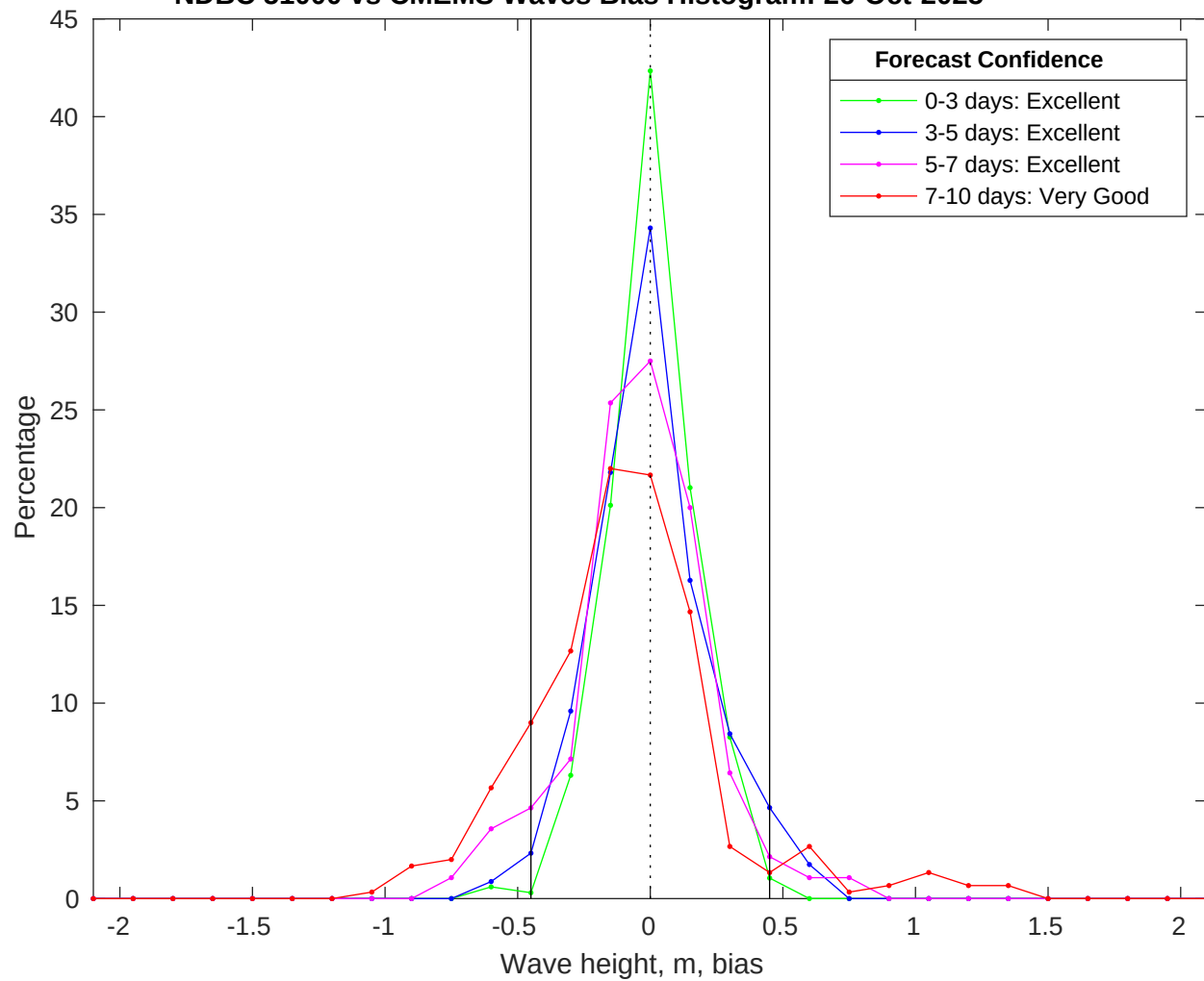
NDBC 51000 vs CMEMS Waves Bias Histogram: 26-Oct-2025
