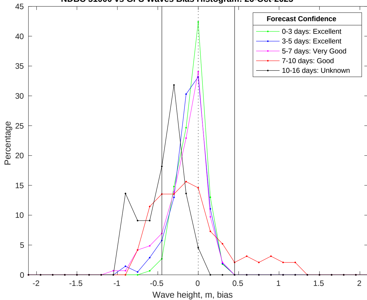
NDBC 51000 vs GFS Waves Bias Histogram: 26-Oct-2025
