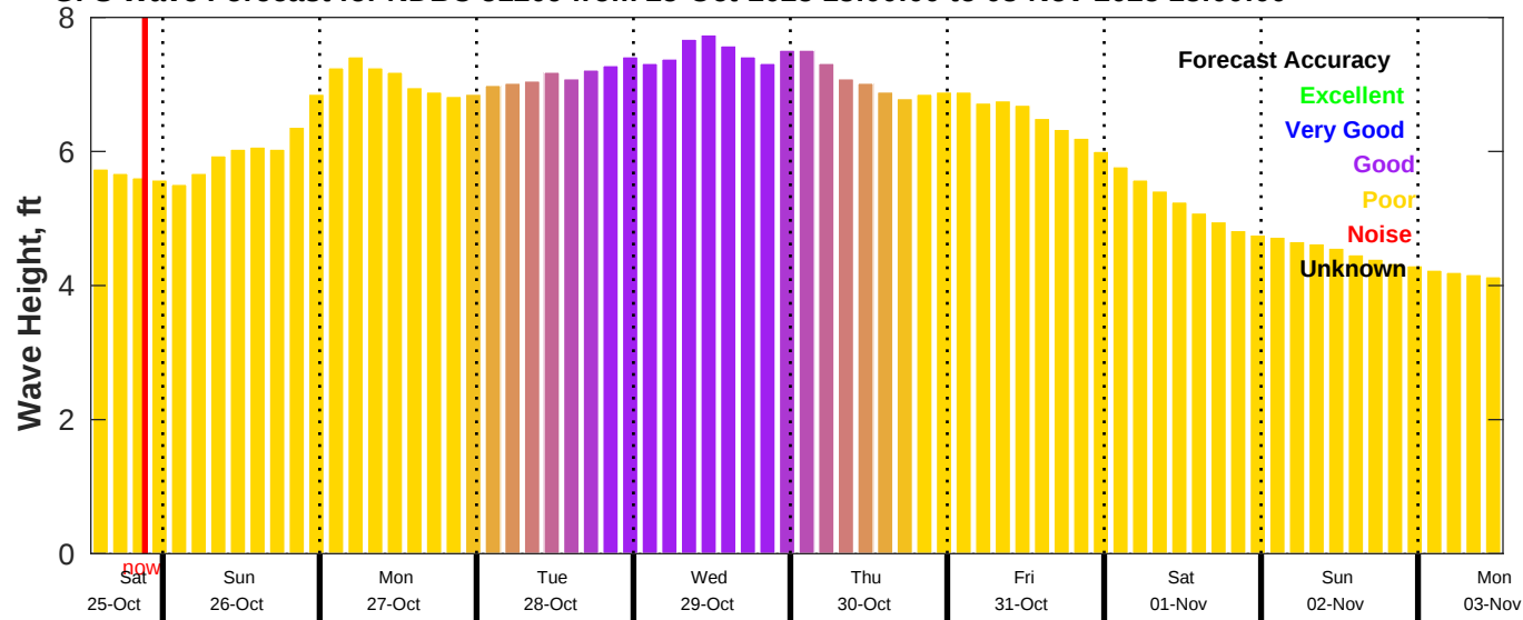
GFS Wave Forecast for NDBC 51209 from 25-Oct-2025 13:00:00 to 03-Nov-2025 13:00:00
