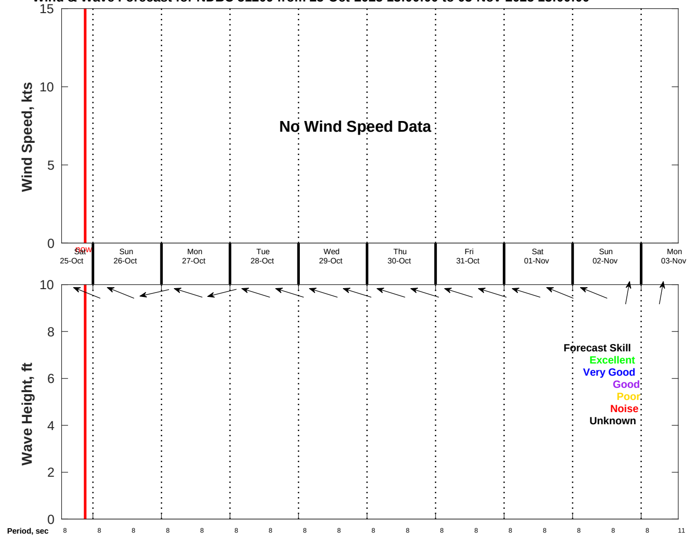
Wind & Wave Forecast for NDBC 51209 from 25-Oct-2025 13:00:00 to 03-Nov-2025 13:00:00
