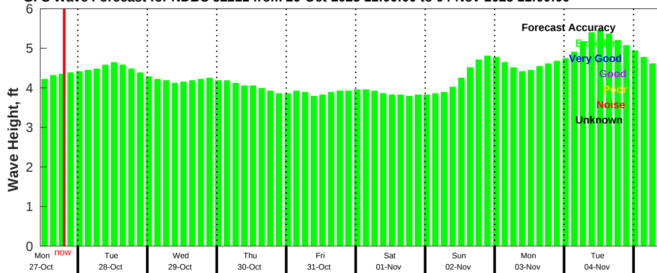
GFS Wave Forecast for NDBC 52211 from 26-Oct-2025 11:00:00 to 04-Nov-2025 11:00:00
