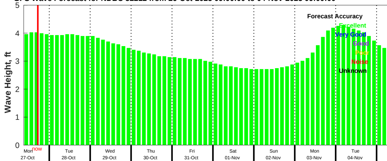
GFS Wave Forecast for NDBC 52212 from 26-Oct-2025 09:00:00 to 04-Nov-2025 09:00:00
