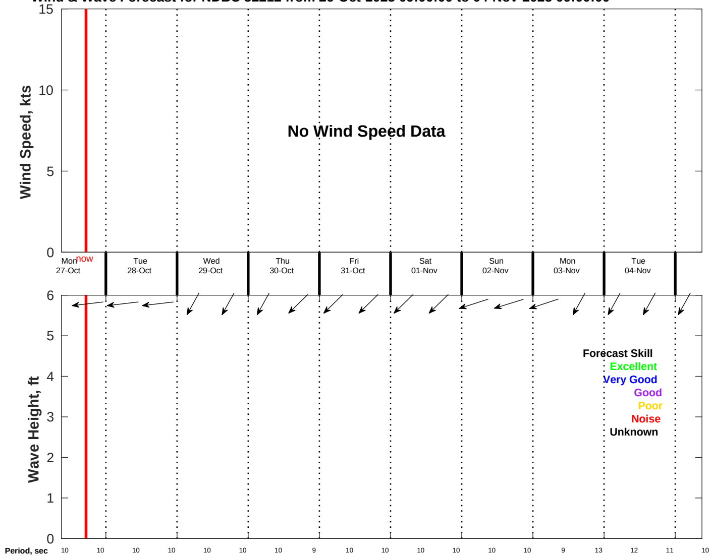
Wind & Wave Forecast for NDBC 52212 from 26-Oct-2025 09:00:00 to 04-Nov-2025 09:00:00
