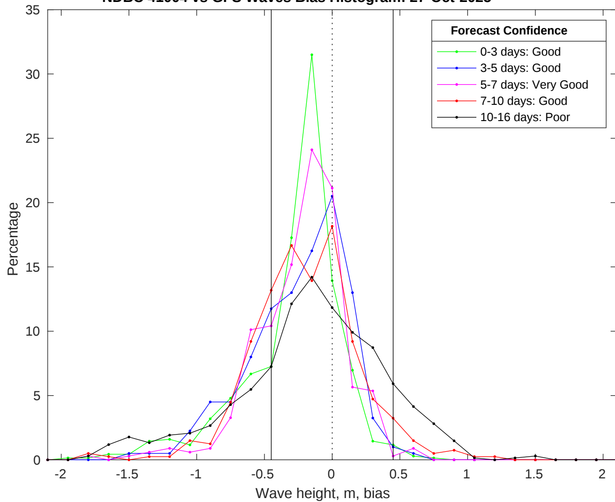
NDBC 41004 vs GFS Waves Bias Histogram: 27-Oct-2025
