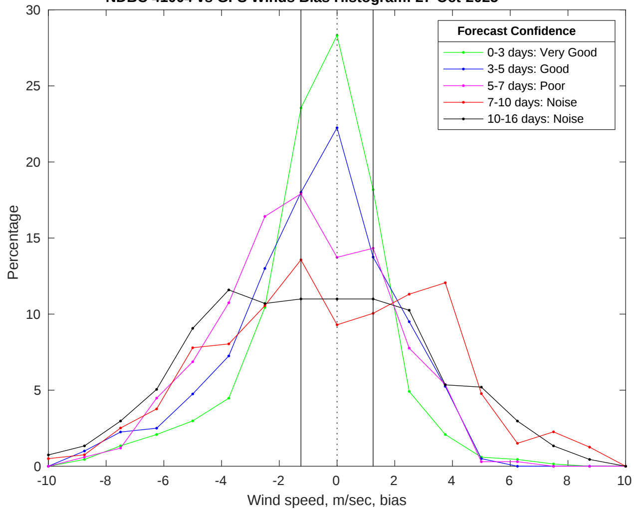
NDBC 41004 vs GFS Winds Bias Histogram: 27-Oct-2025
