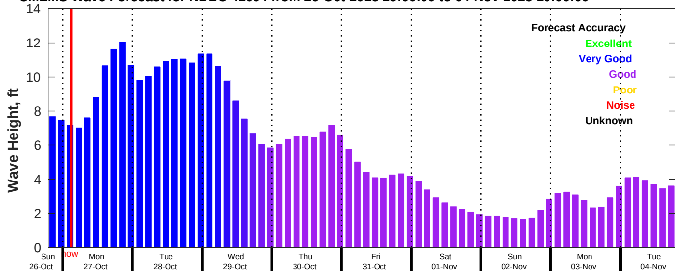
CMEMS Wave Forecast for NDBC 41004 from 26-Oct-2025 19:00:00 to 04-Nov-2025 19:00:00
