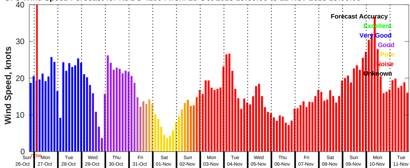
GFS Wind Speed Forecast for NDBC 41004 from 26-Oct-2025 19:00:00 to 11-Nov-2025 19:00:00
