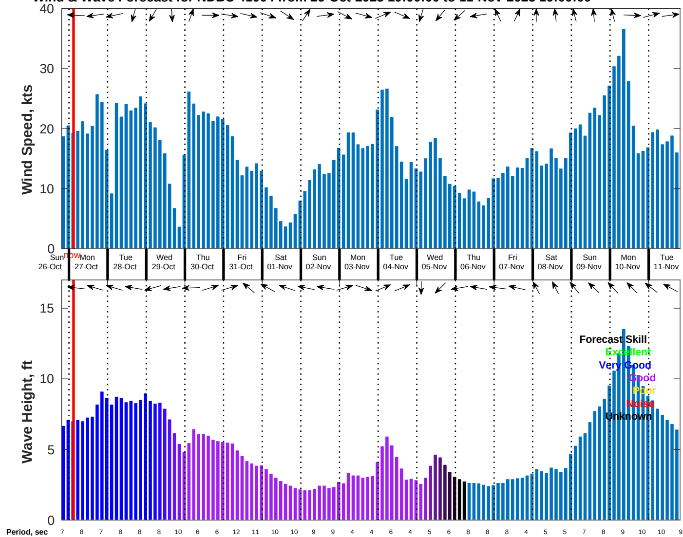
Wind & Wave Forecast for NDBC 41004 from 26-Oct-2025 19:00:00 to 11-Nov-2025 19:00:00
