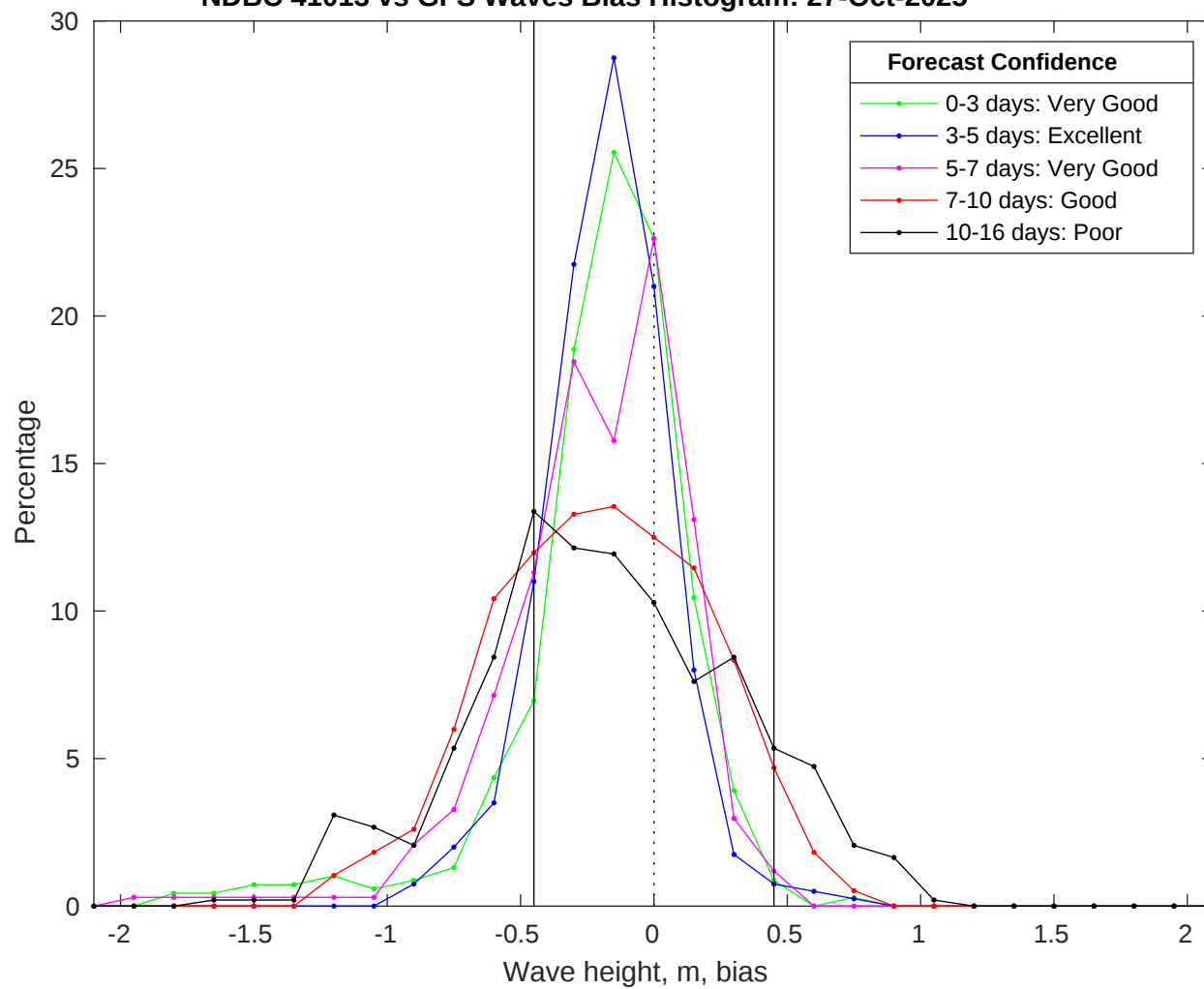
NDBC 41013 vs GFS Waves Bias Histogram: 27-Oct-2025
