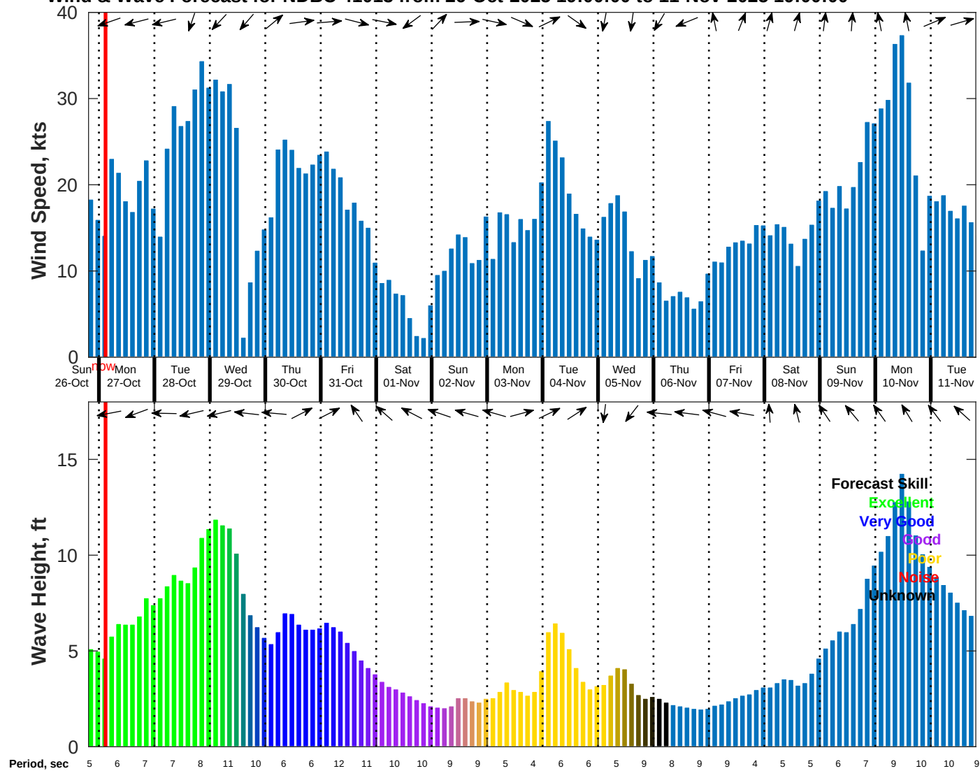
Wind & Wave Forecast for NDBC 41013 from 26-Oct-2025 19:00:00 to 11-Nov-2025 19:00:00
